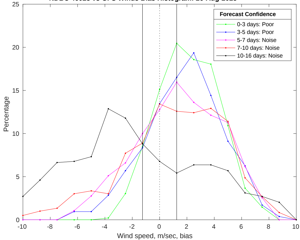
NDBC 46028 vs GFS Winds Bias Histogram: 26-Aug-2025
