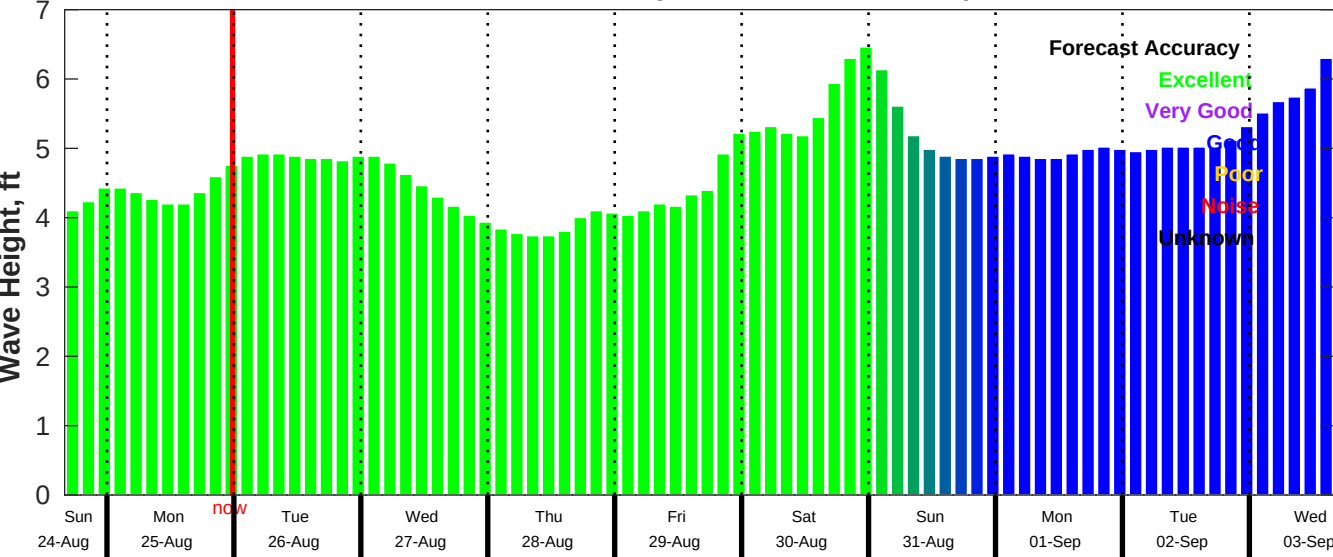
CMEMS Wave Forecast for NDBC 46028 from 24-Aug-2025 16:00:00 to 03-Sep-2025 16:00:00
