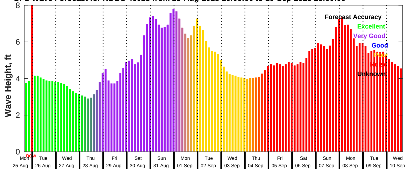
GFS Wave Forecast for NDBC 46028 from 25-Aug-2025 16:00:00 to 10-Sep-2025 16:00:00
