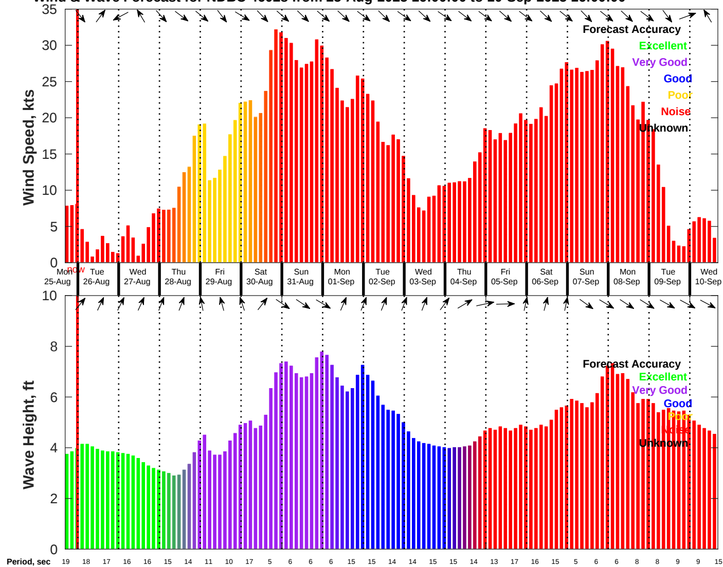
Wind & Wave Forecast for NDBC 46028 from 25-Aug-2025 16:00:00 to 10-Sep-2025 16:00:00
