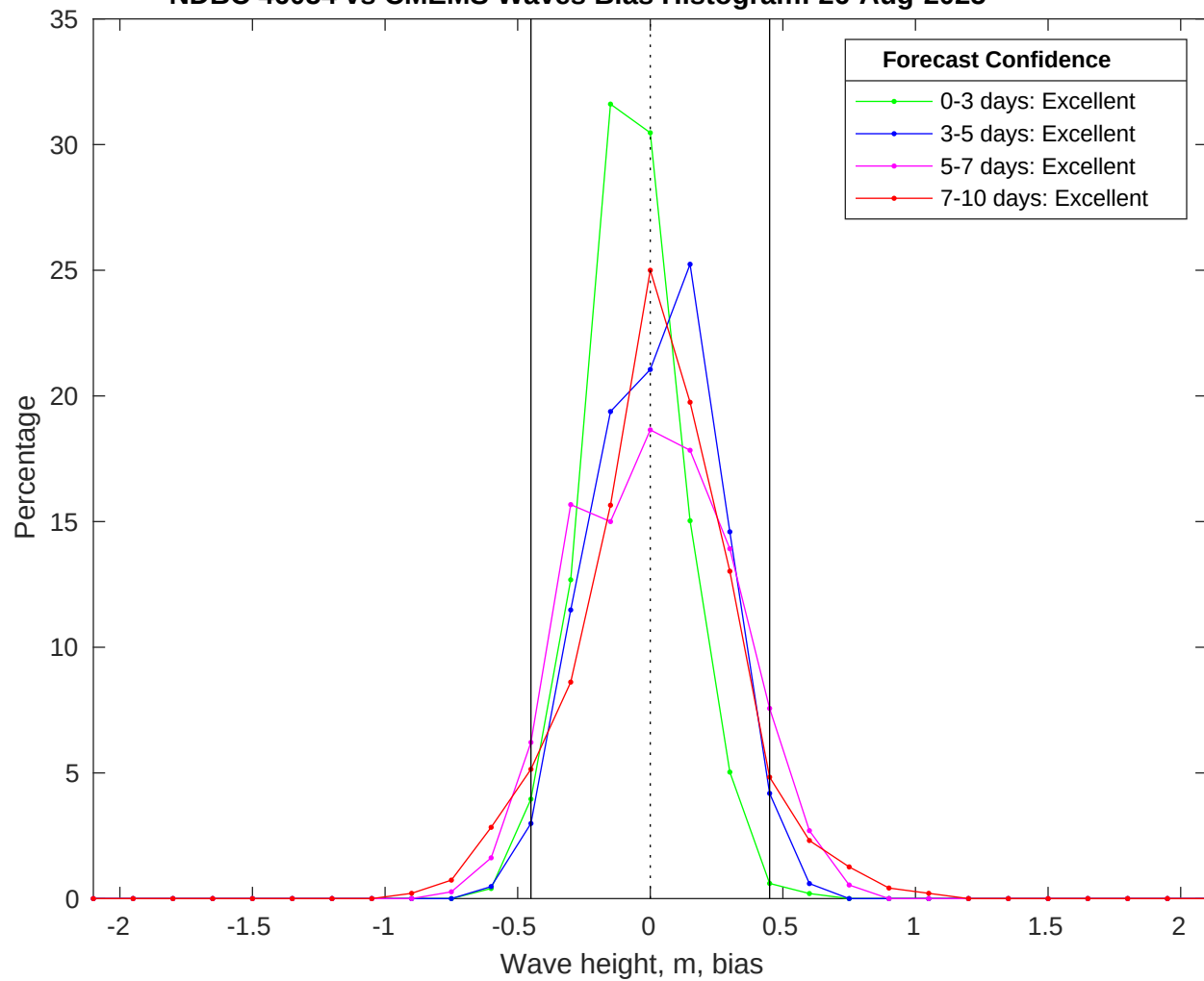
NDBC 46054 vs CMEMS Waves Bias Histogram: 26-Aug-2025
