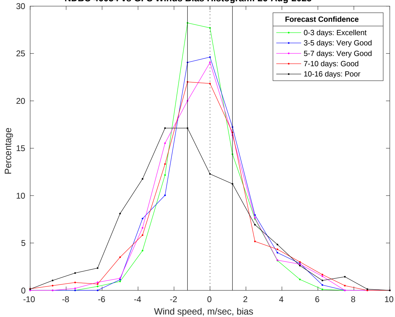
NDBC 46054 vs GFS Winds Bias Histogram: 26-Aug-2025
