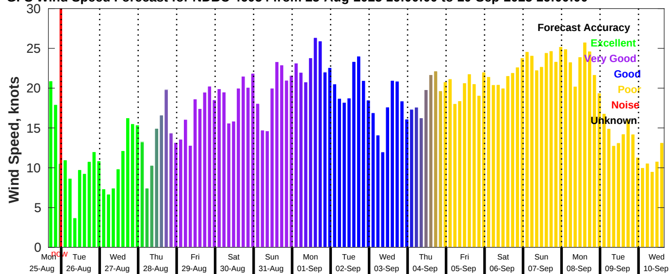
GFS Wind Speed Forecast for NDBC 46054 from 25-Aug-2025 16:00:00 to 10-Sep-2025 16:00:00
