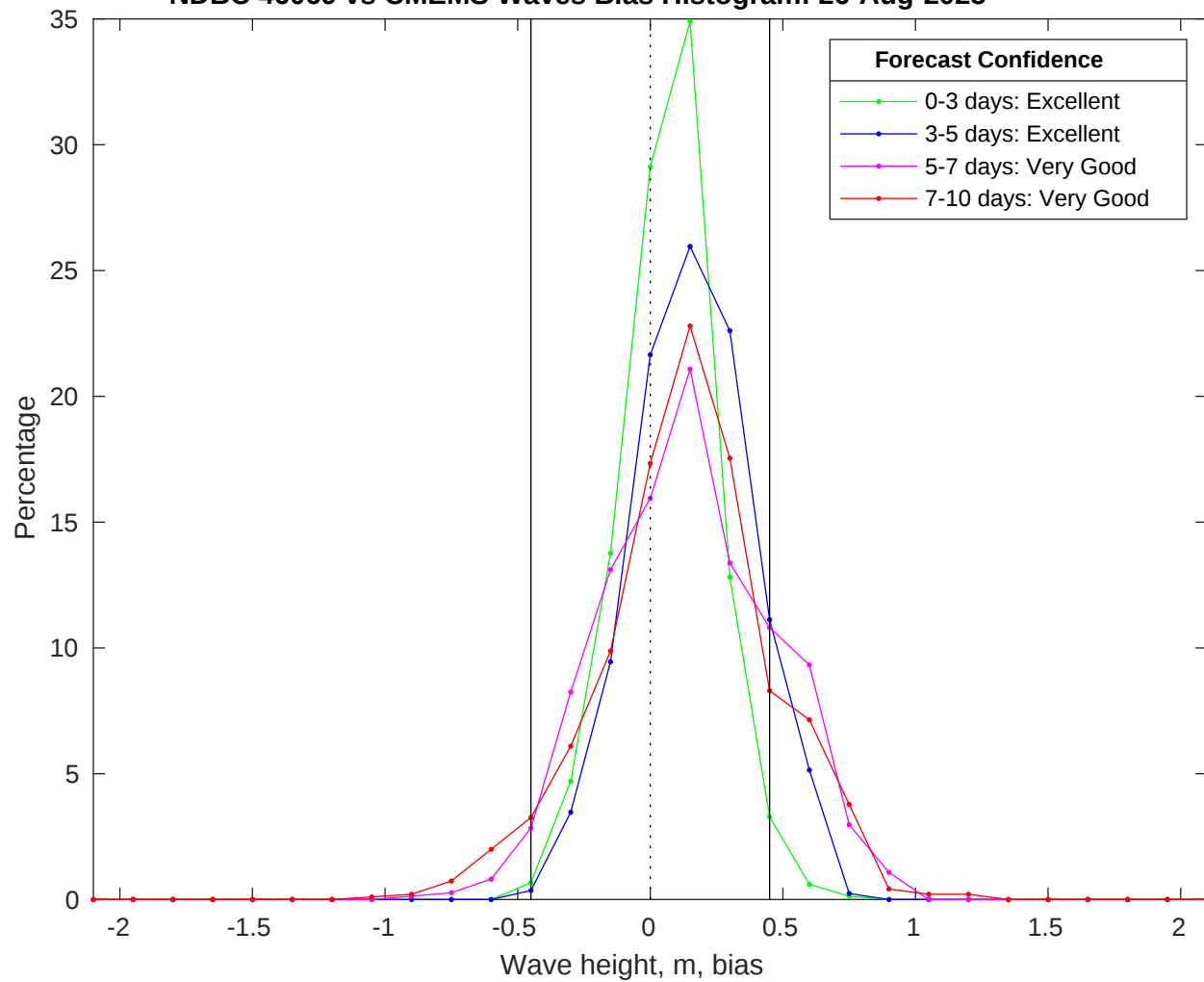
NDBC 46069 vs CMEMS Waves Bias Histogram: 26-Aug-2025
