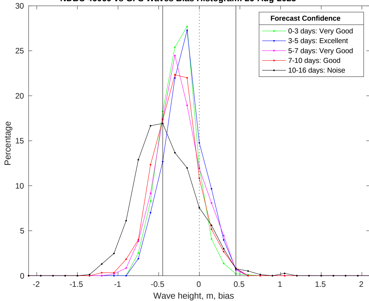
NDBC 46069 vs GFS Waves Bias Histogram: 26-Aug-2025
