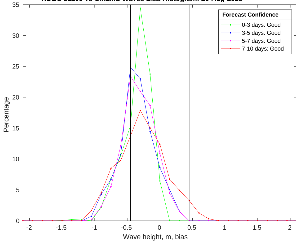
NDBC 51209 vs CMEMS Waves Bias Histogram: 26-Aug-2025
