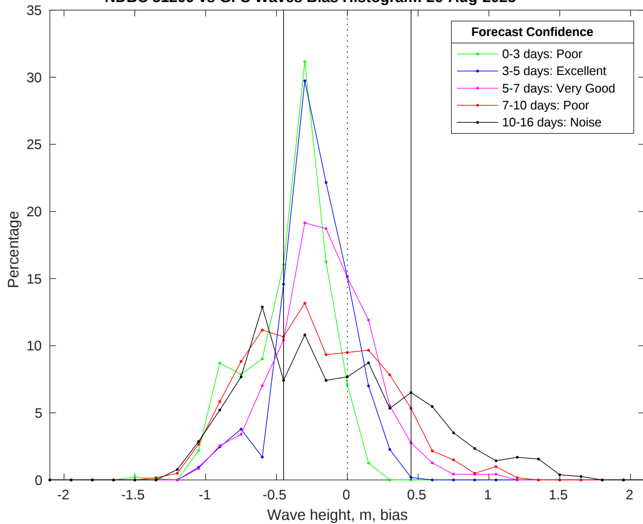
NDBC 51209 vs GFS Waves Bias Histogram: 26-Aug-2025
