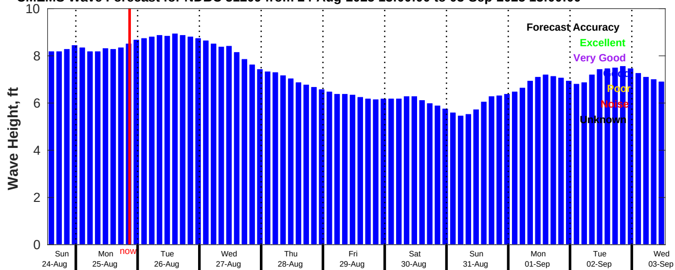
CMEMS Wave Forecast for NDBC 51209 from 24-Aug-2025 13:00:00 to 03-Sep-2025 13:00:00
