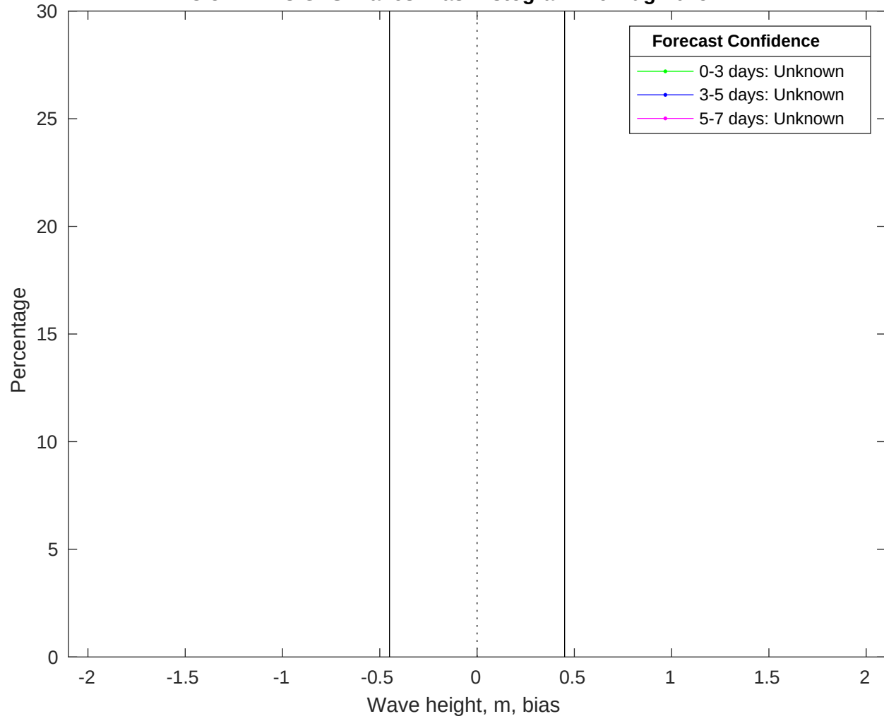
NDBC 51211 vs GFS Waves Bias Histogram: 26-Aug-2025
