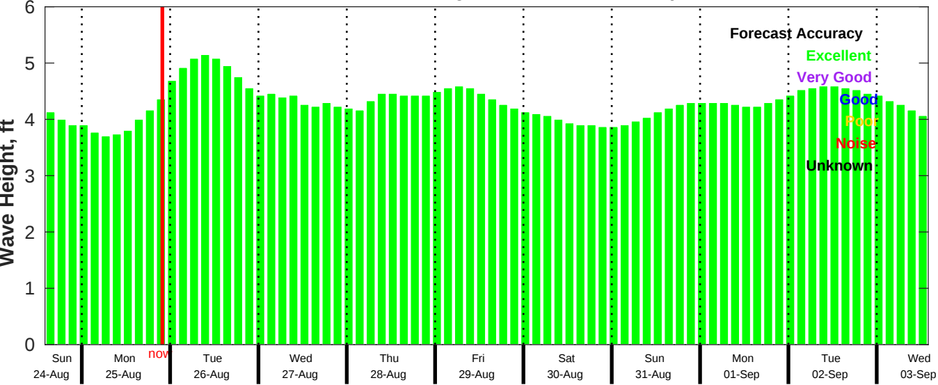
CMEMS Wave Forecast for NDBC 51211 from 24-Aug-2025 14:00:00 to 03-Sep-2025 14:00:00
