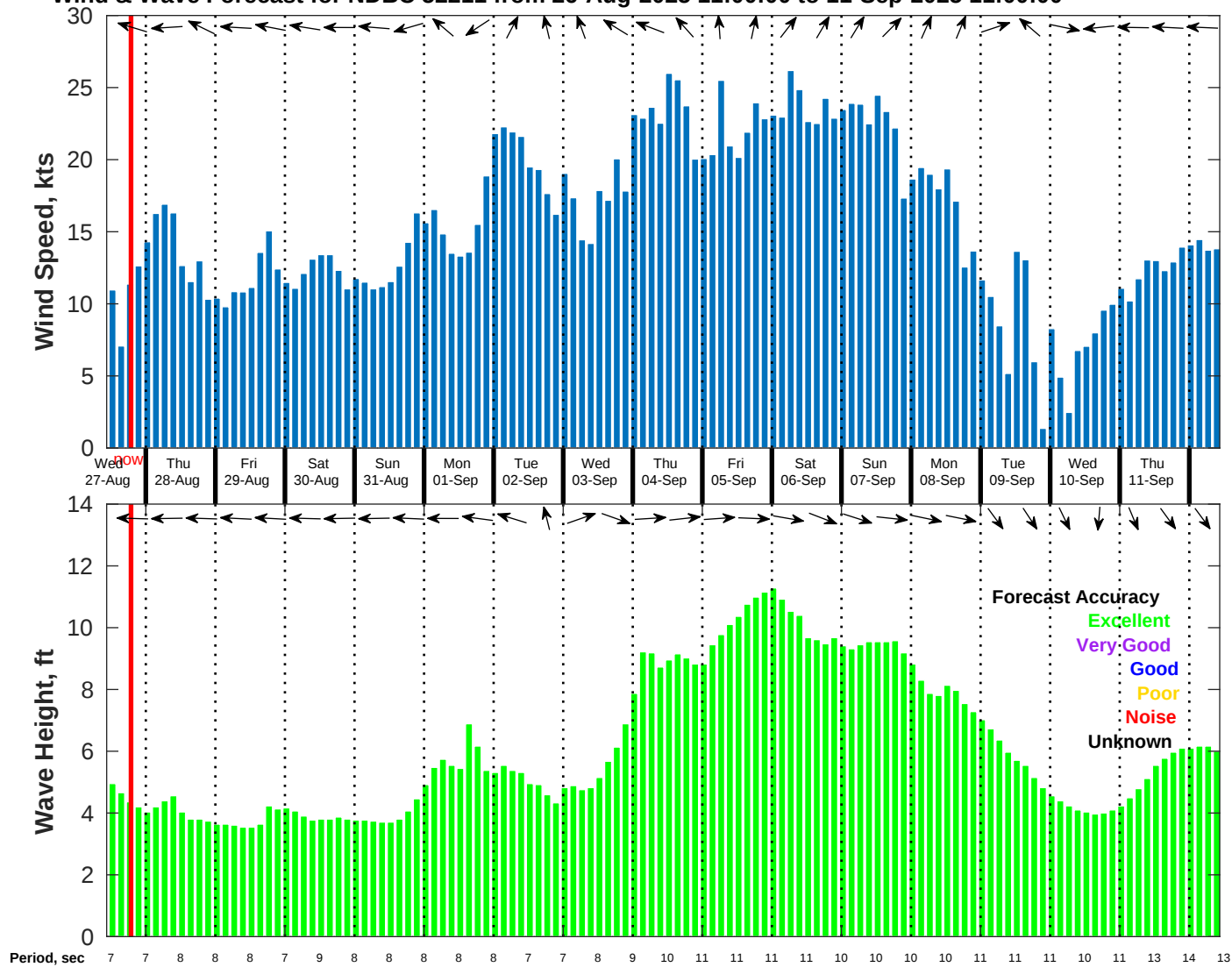
Wind & Wave Forecast for NDBC 52211 from 26-Aug-2025 11:00:00 to 11-Sep-2025 11:00:00
