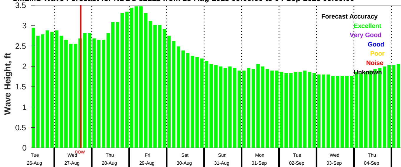
CMEMS Wave Forecast for NDBC 52212 from 25-Aug-2025 09:00:00 to 04-Sep-2025 09:00:00
