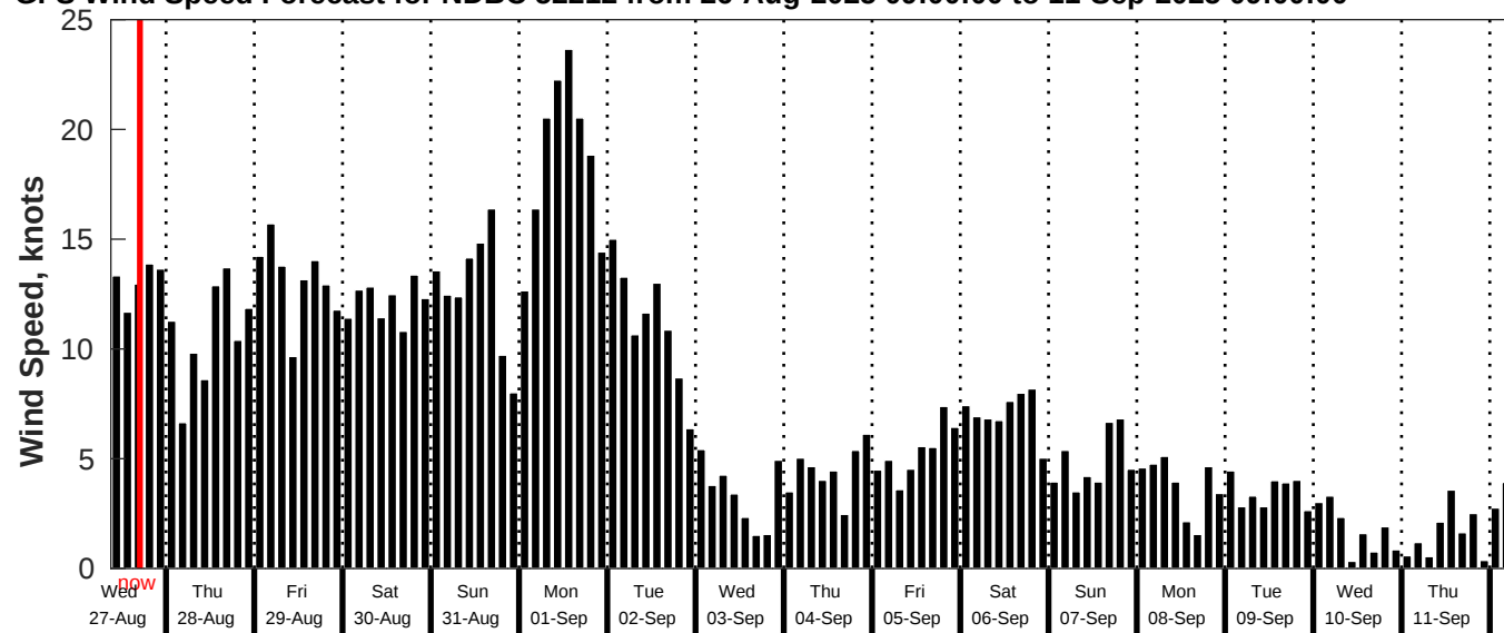
GFS Wind Speed Forecast for NDBC 52212 from 26-Aug-2025 09:00:00 to 11-Sep-2025 09:00:00
