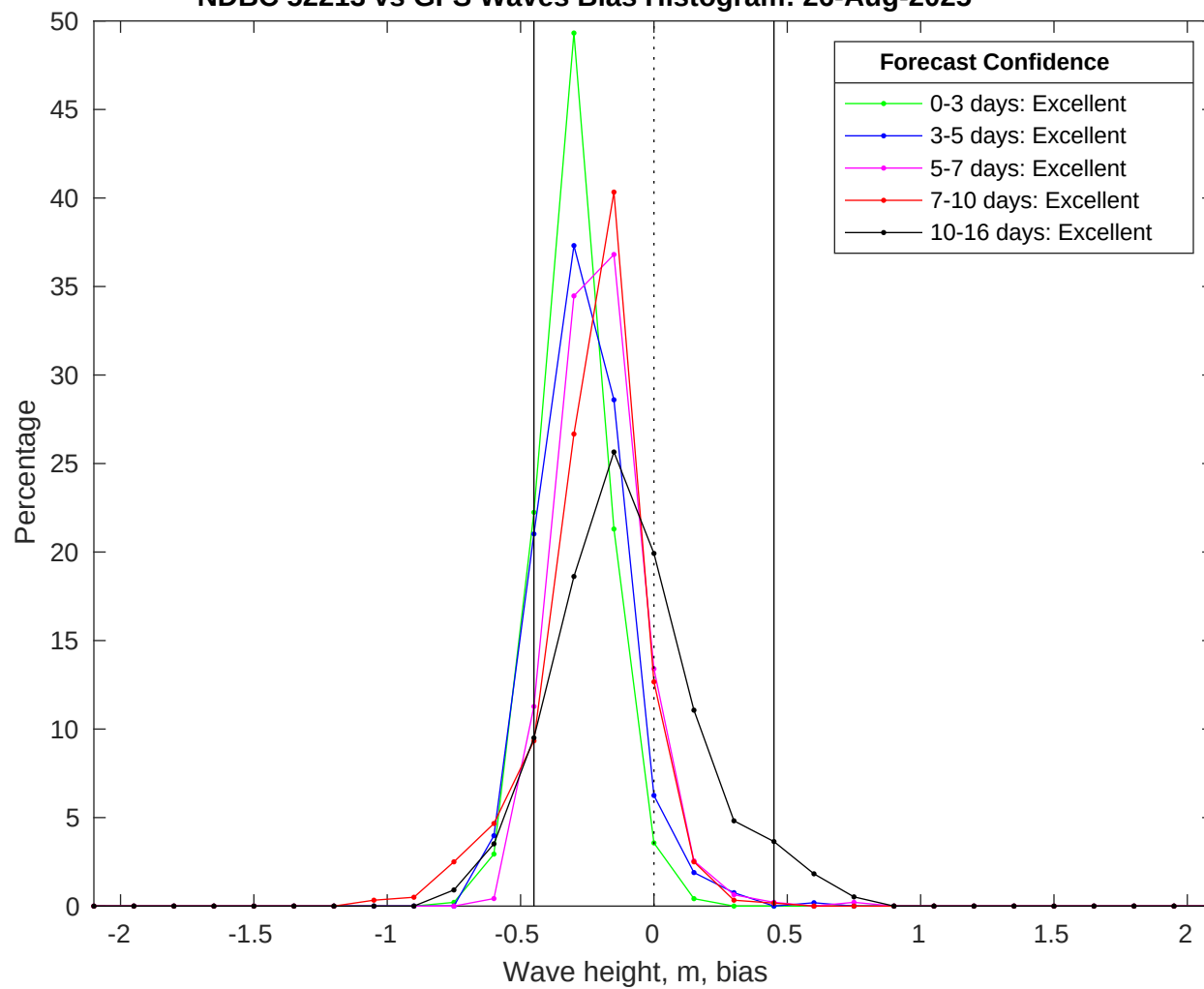
NDBC 52213 vs GFS Waves Bias Histogram: 26-Aug-2025
