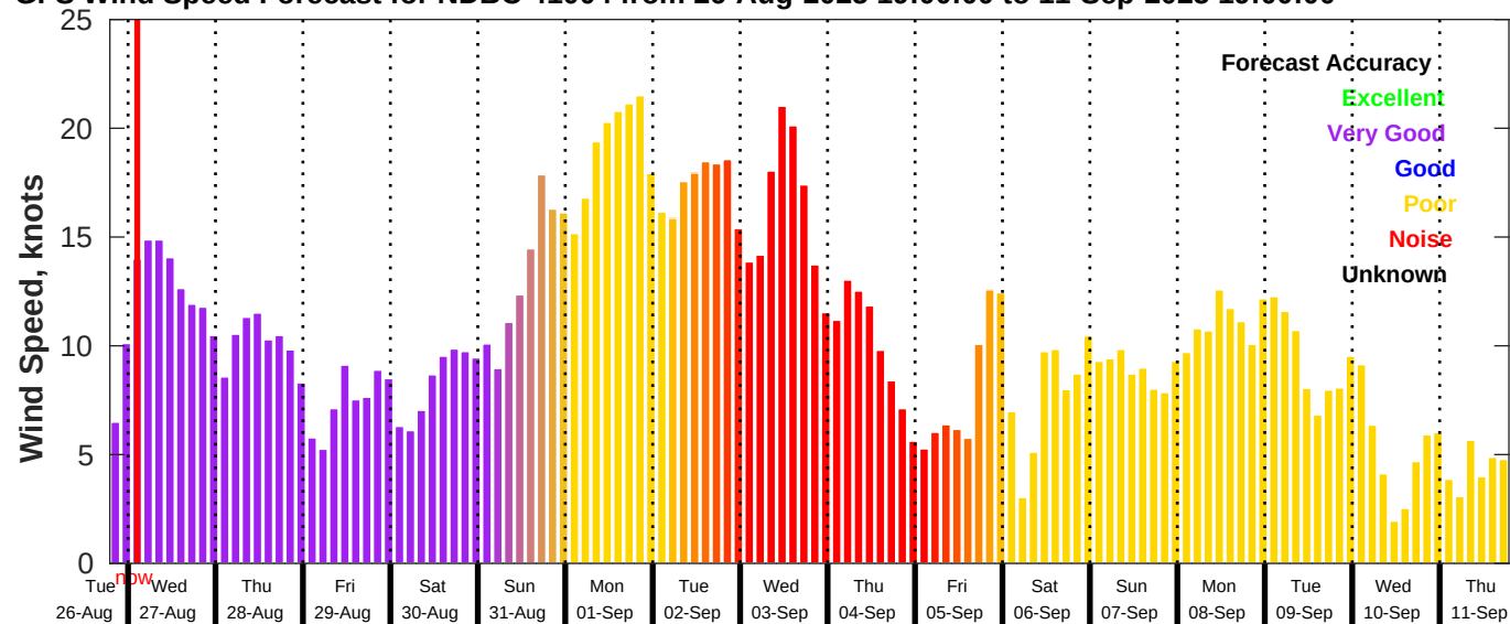
GFS Wind Speed Forecast for NDBC 41004 from 26-Aug-2025 19:00:00 to 11-Sep-2025 19:00:00
