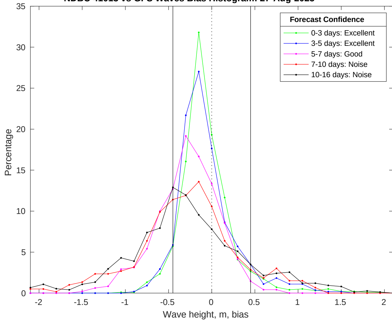
NDBC 41013 vs GFS Waves Bias Histogram: 27-Aug-2025
