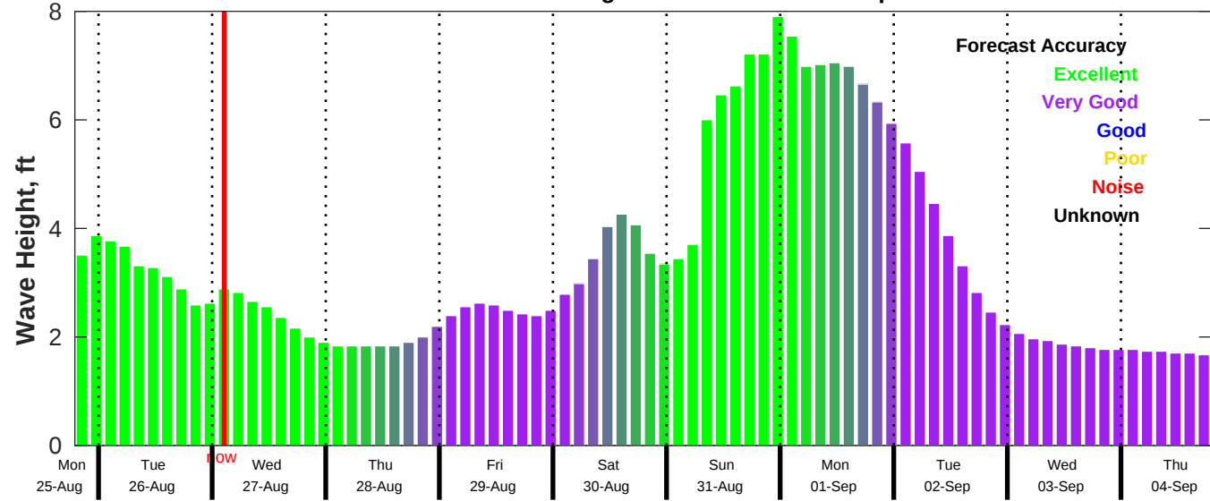
CMEMS Wave Forecast for NDBC 41013 from 25-Aug-2025 19:00:00 to 04-Sep-2025 19:00:00
