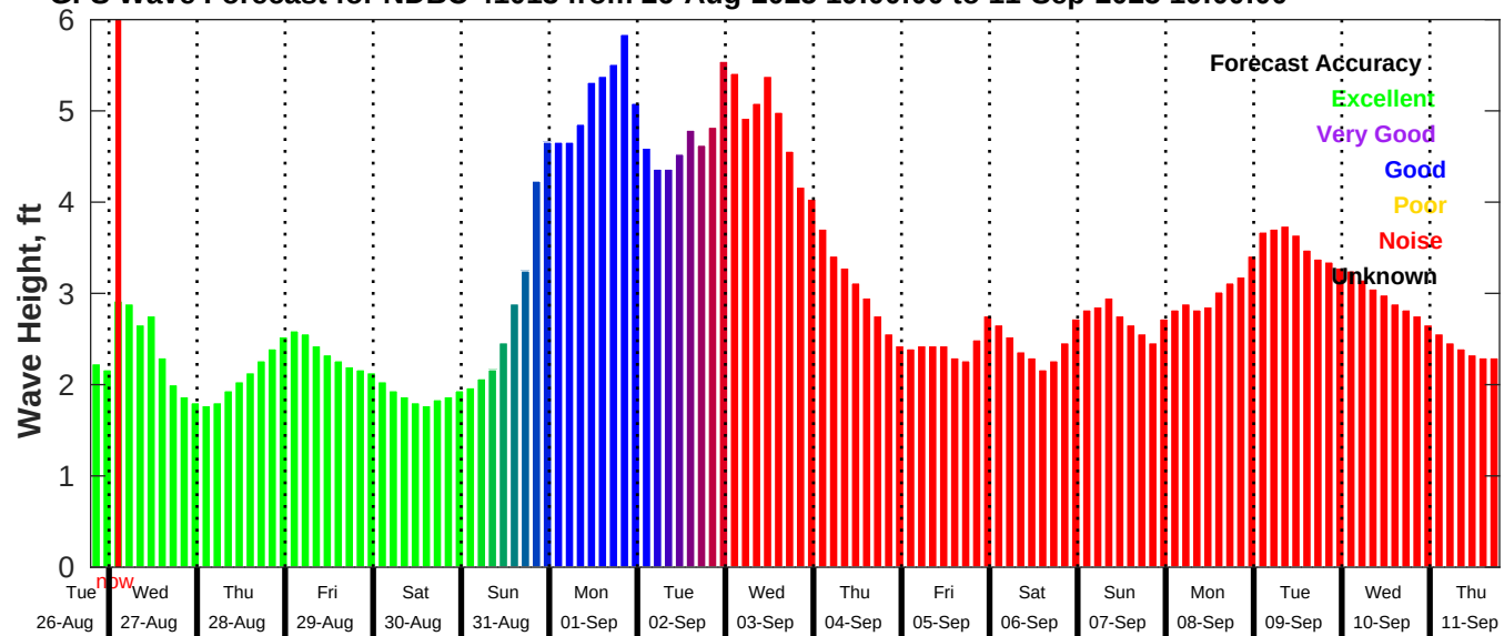
GFS Wave Forecast for NDBC 41013 from 26-Aug-2025 19:00:00 to 11-Sep-2025 19:00:00
