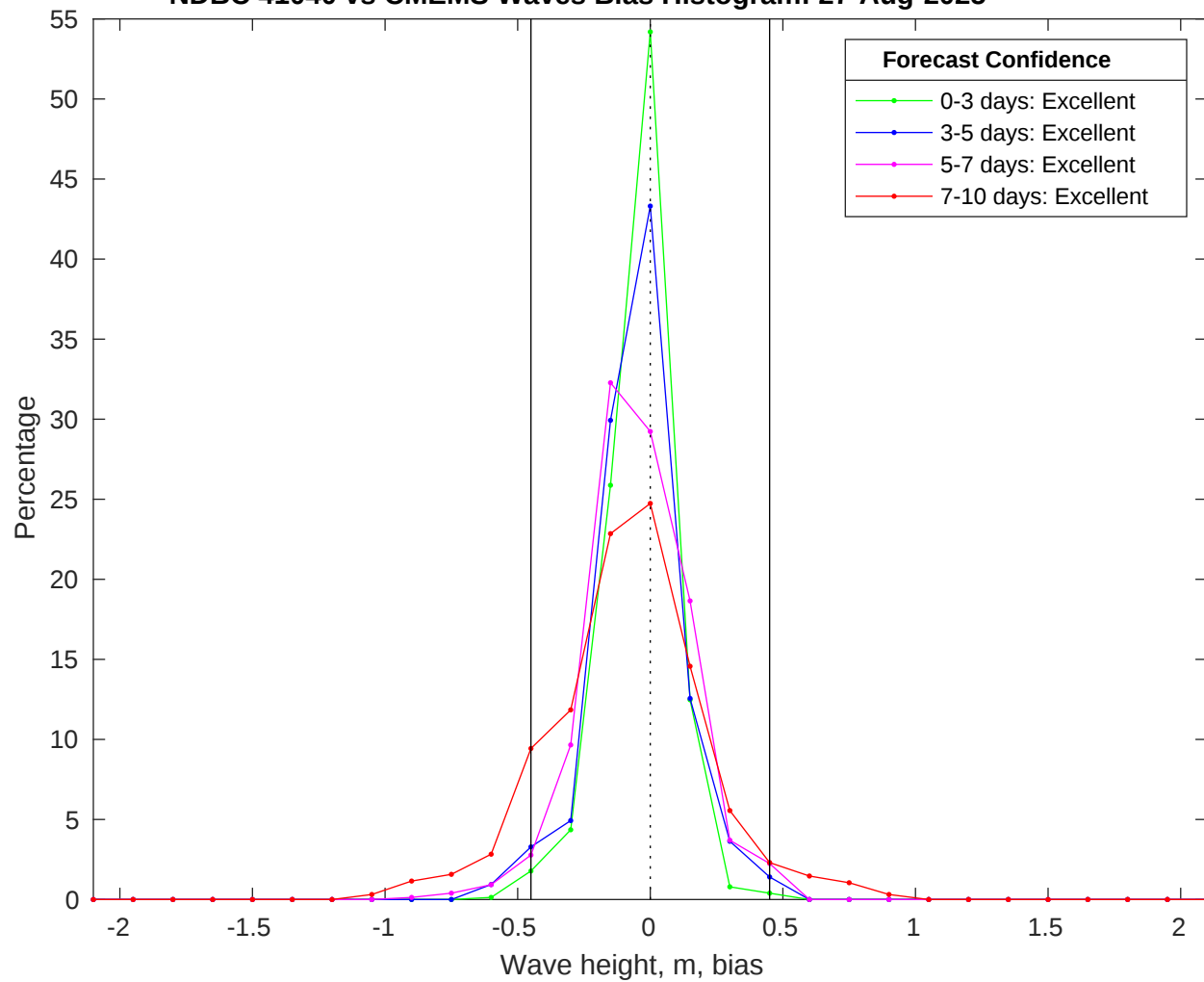
NDBC 41040 vs CMEMS Waves Bias Histogram: 27-Aug-2025
