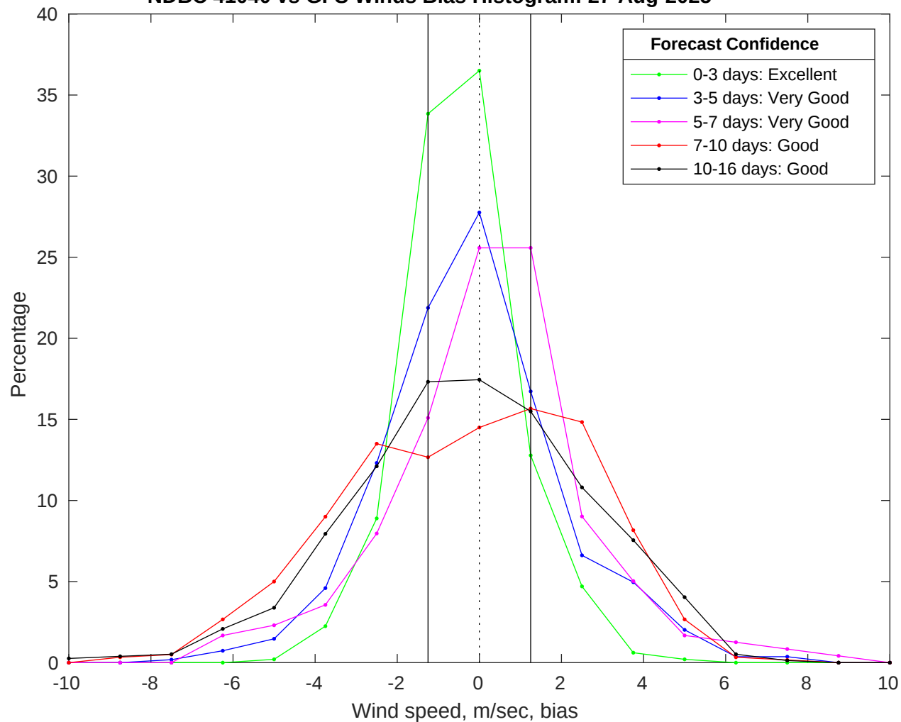
NDBC 41040 vs GFS Winds Bias Histogram: 27-Aug-2025
