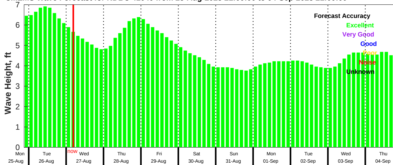
CMEMS Wave Forecast for NDBC 41040 from 25-Aug-2025 21:00:00 to 04-Sep-2025 21:00:00
