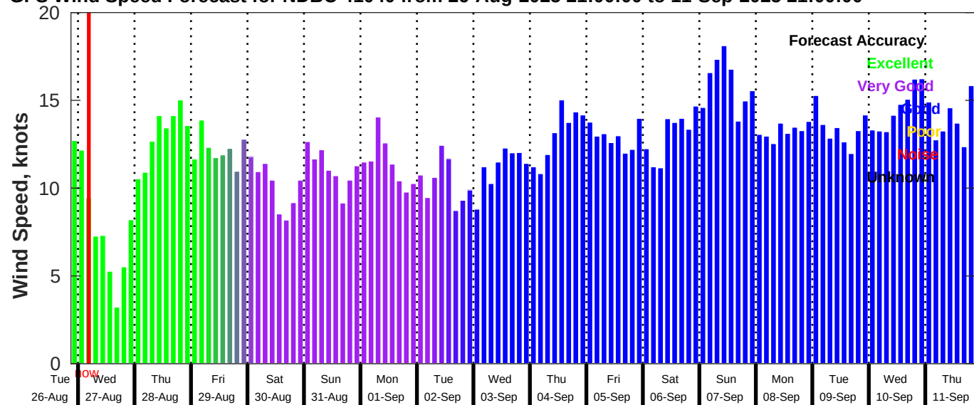
GFS Wind Speed Forecast for NDBC 41040 from 26-Aug-2025 21:00:00 to 11-Sep-2025 21:00:00
