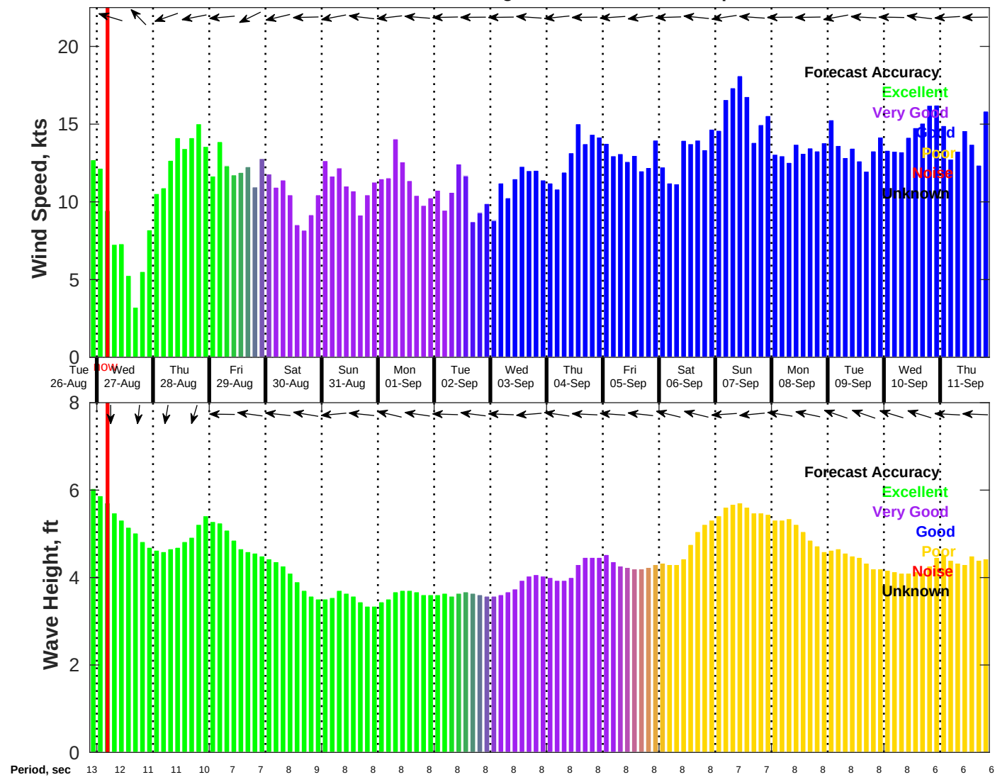
Wind & Wave Forecast for NDBC 41040 from 26-Aug-2025 21:00:00 to 11-Sep-2025 21:00:00
