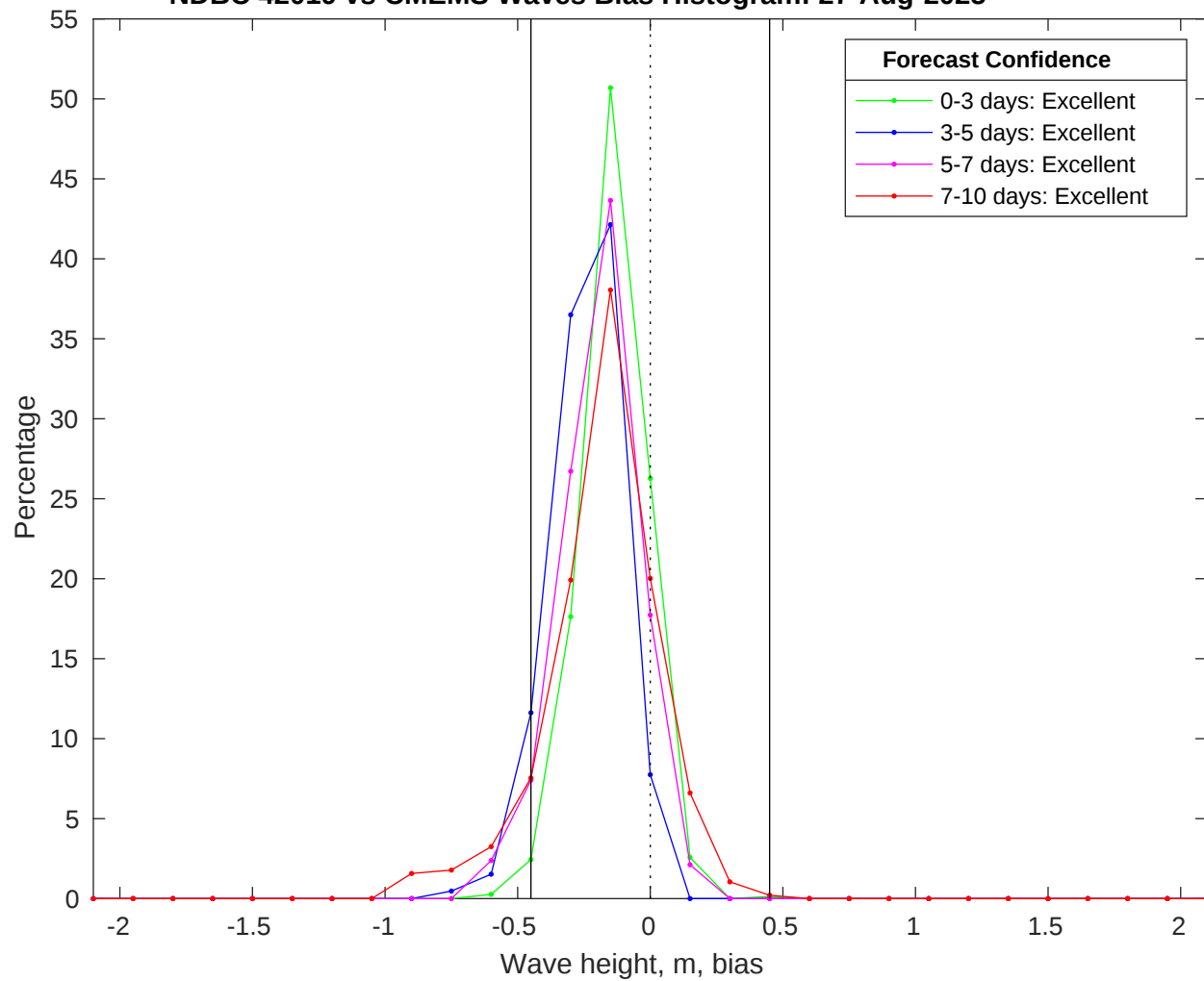
NDBC 42019 vs CMEMS Waves Bias Histogram: 27-Aug-2025
