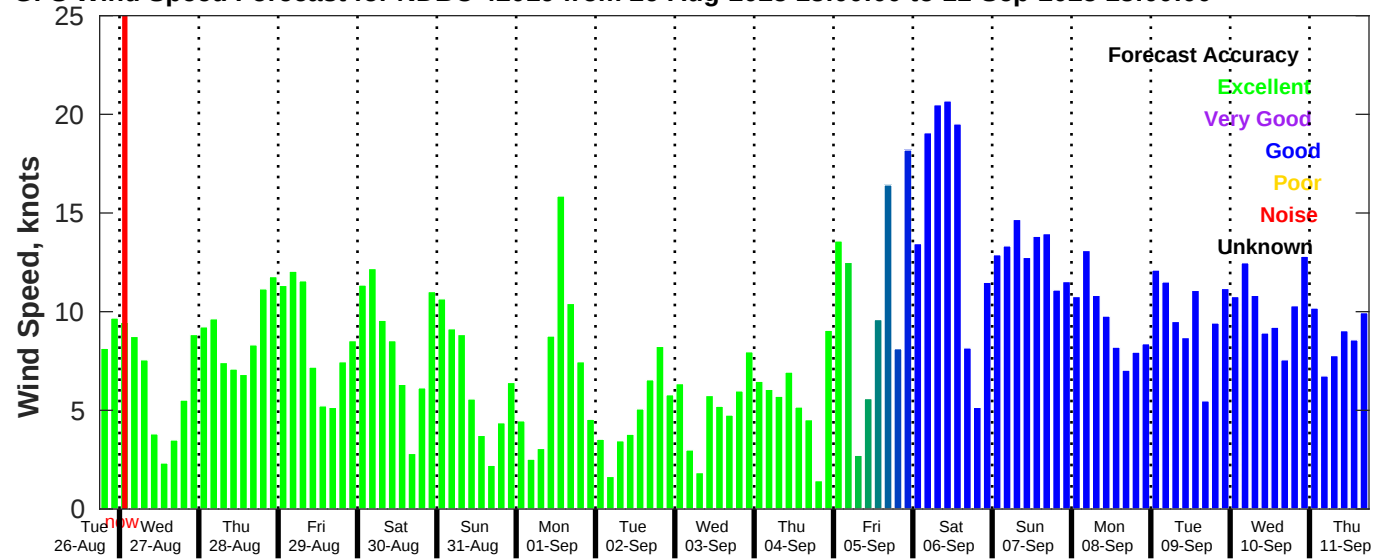
GFS Wind Speed Forecast for NDBC 42019 from 26-Aug-2025 18:00:00 to 11-Sep-2025 18:00:00
