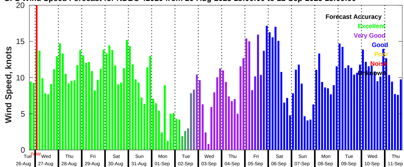
GFS Wind Speed Forecast for NDBC 42020 from 26-Aug-2025 18:00:00 to 11-Sep-2025 18:00:00
