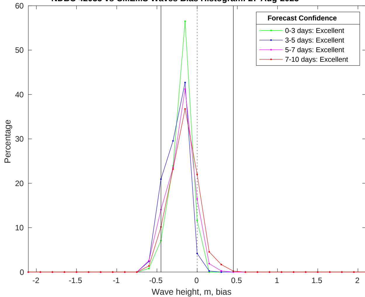
NDBC 42035 vs CMEMS Waves Bias Histogram: 27-Aug-2025
