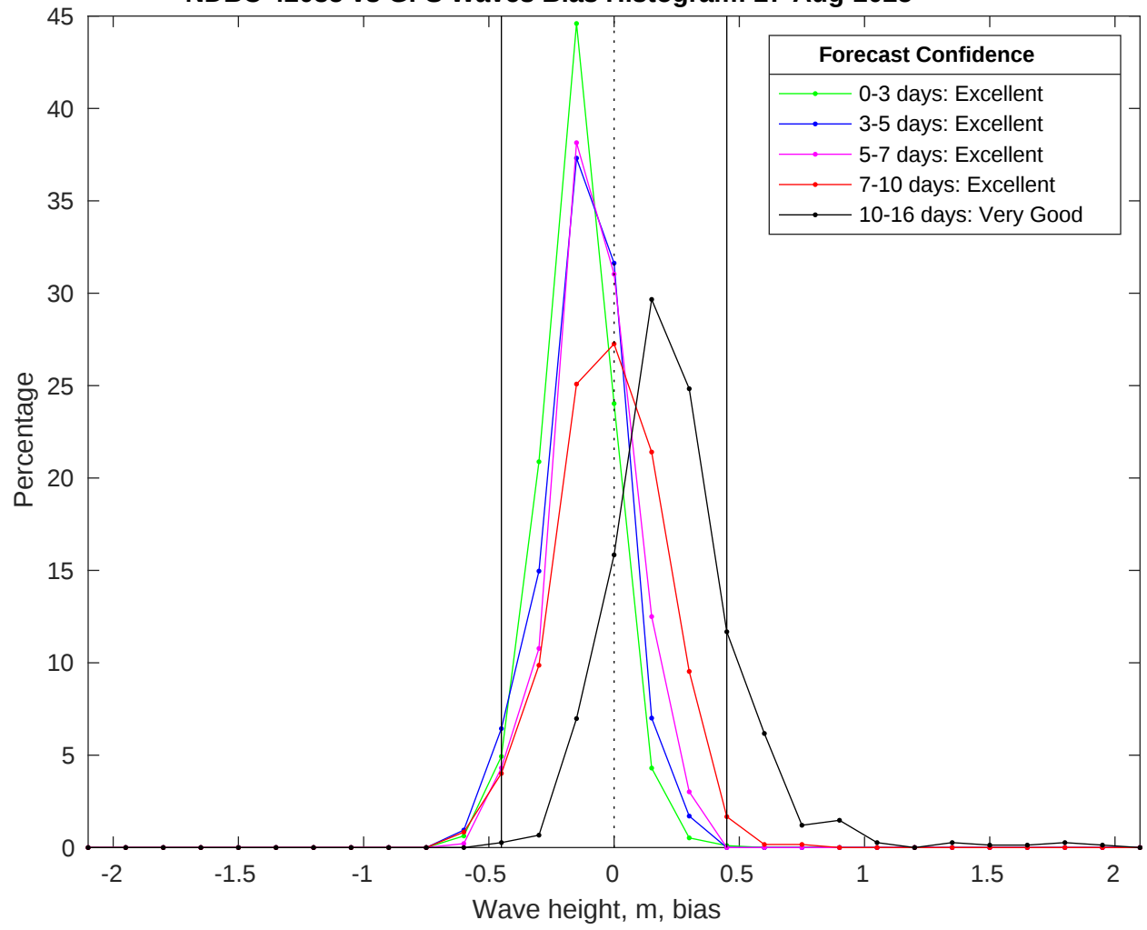
NDBC 42035 vs GFS Waves Bias Histogram: 27-Aug-2025
