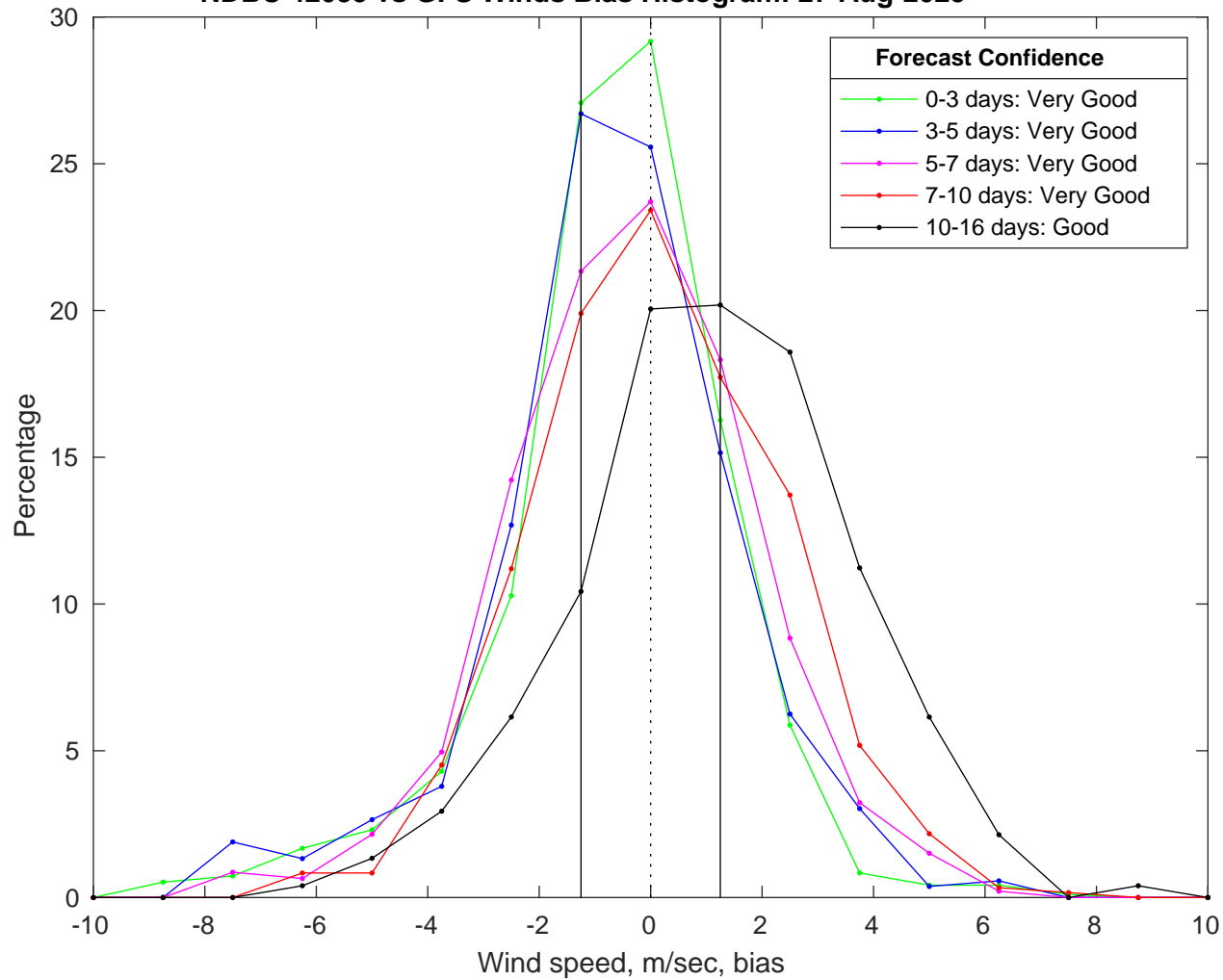
NDBC 42035 vs GFS Winds Bias Histogram: 27-Aug-2025
