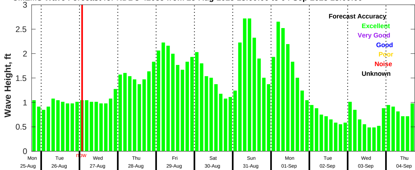
CMEMS Wave Forecast for NDBC 42035 from 25-Aug-2025 18:00:00 to 04-Sep-2025 18:00:00
