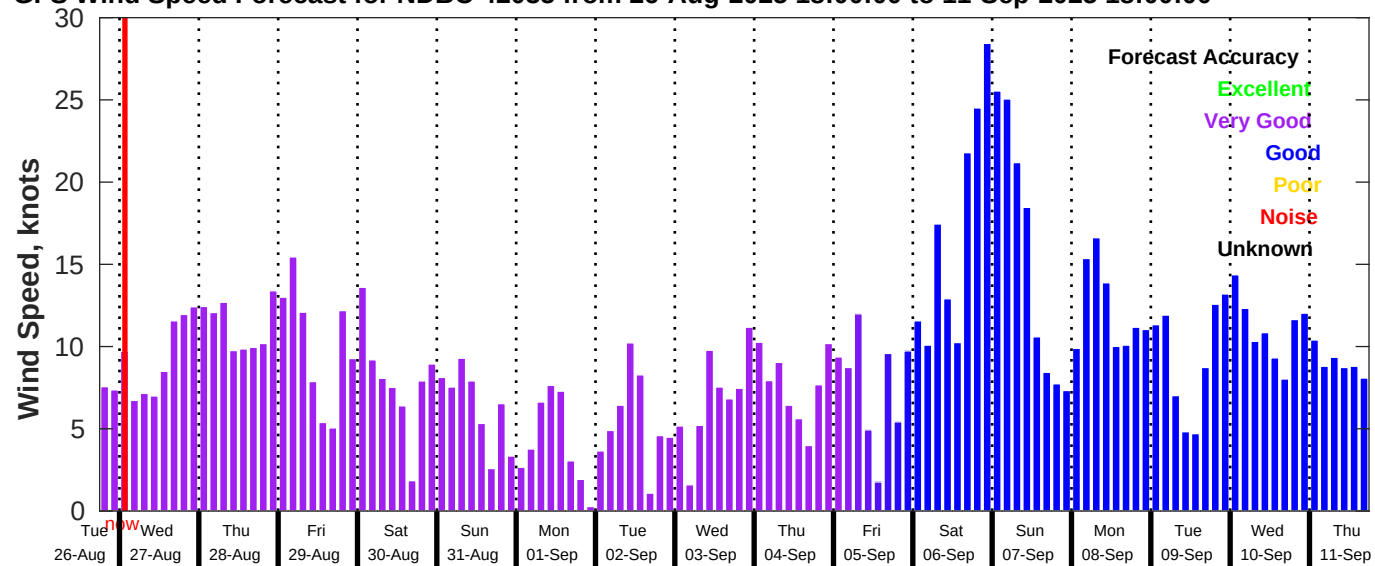
GFS Wind Speed Forecast for NDBC 42035 from 26-Aug-2025 18:00:00 to 11-Sep-2025 18:00:00
