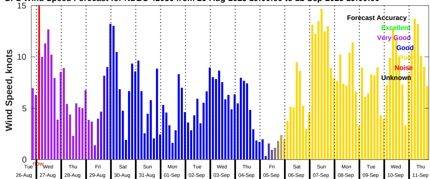
GFS Wind Speed Forecast for NDBC 42036 from 26-Aug-2025 19:00:00 to 11-Sep-2025 19:00:00
