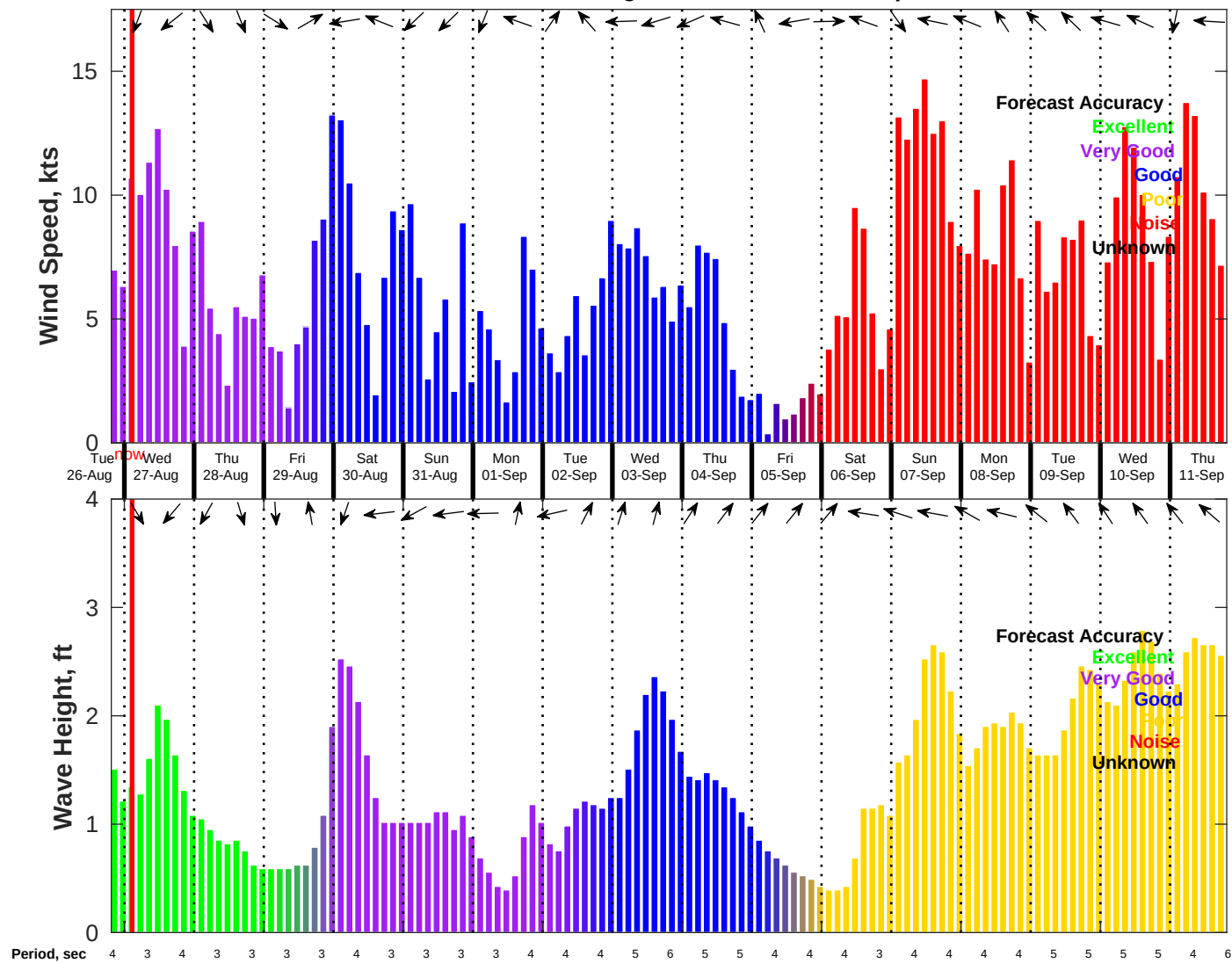
Wind & Wave Forecast for NDBC 42036 from 26-Aug-2025 19:00:00 to 11-Sep-2025 19:00:00
