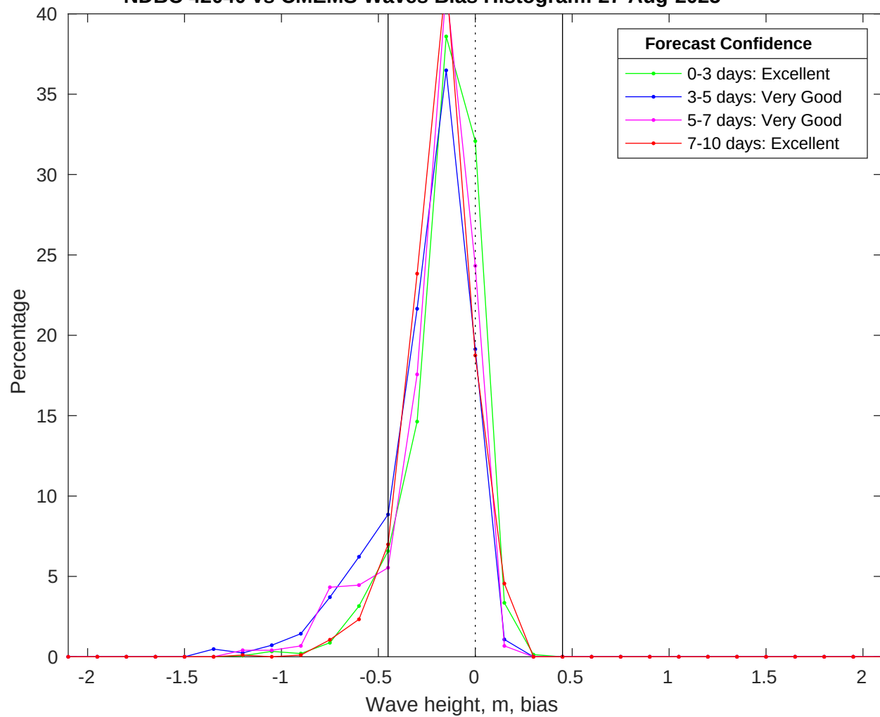
NDBC 42040 vs CMEMS Waves Bias Histogram: 27-Aug-2025
