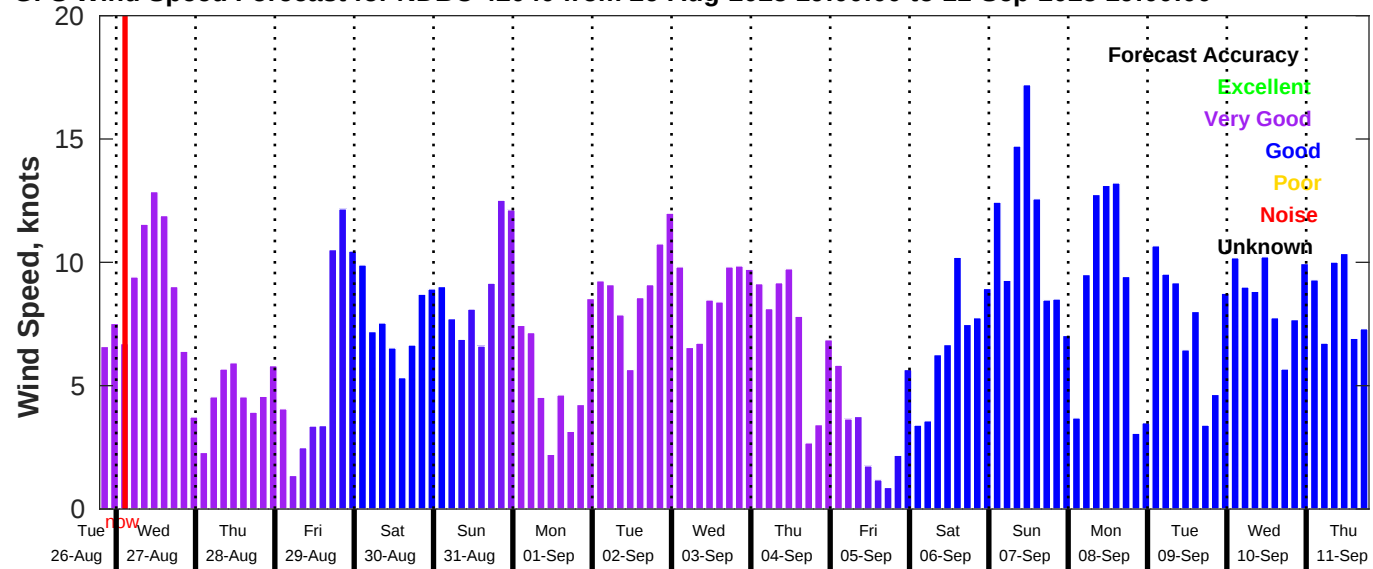
GFS Wind Speed Forecast for NDBC 42040 from 26-Aug-2025 19:00:00 to 11-Sep-2025 19:00:00
