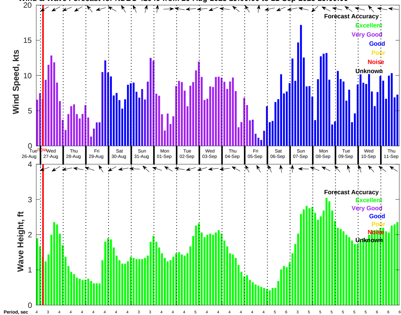
Wind & Wave Forecast for NDBC 42040 from 26-Aug-2025 19:00:00 to 11-Sep-2025 19:00:00
