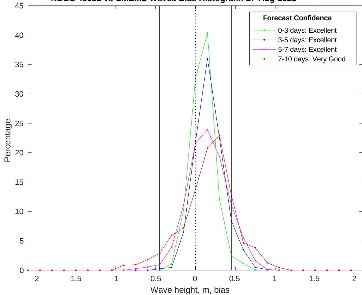
NDBC 46011 vs CMEMS Waves Bias Histogram: 27-Aug-2025
