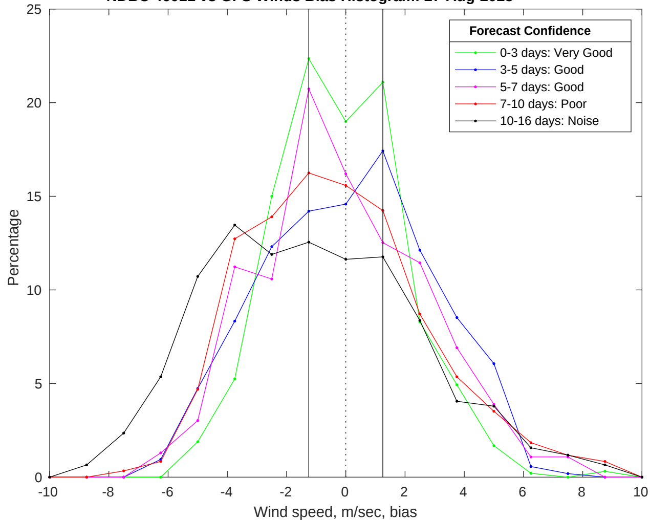
NDBC 46011 vs GFS Winds Bias Histogram: 27-Aug-2025
