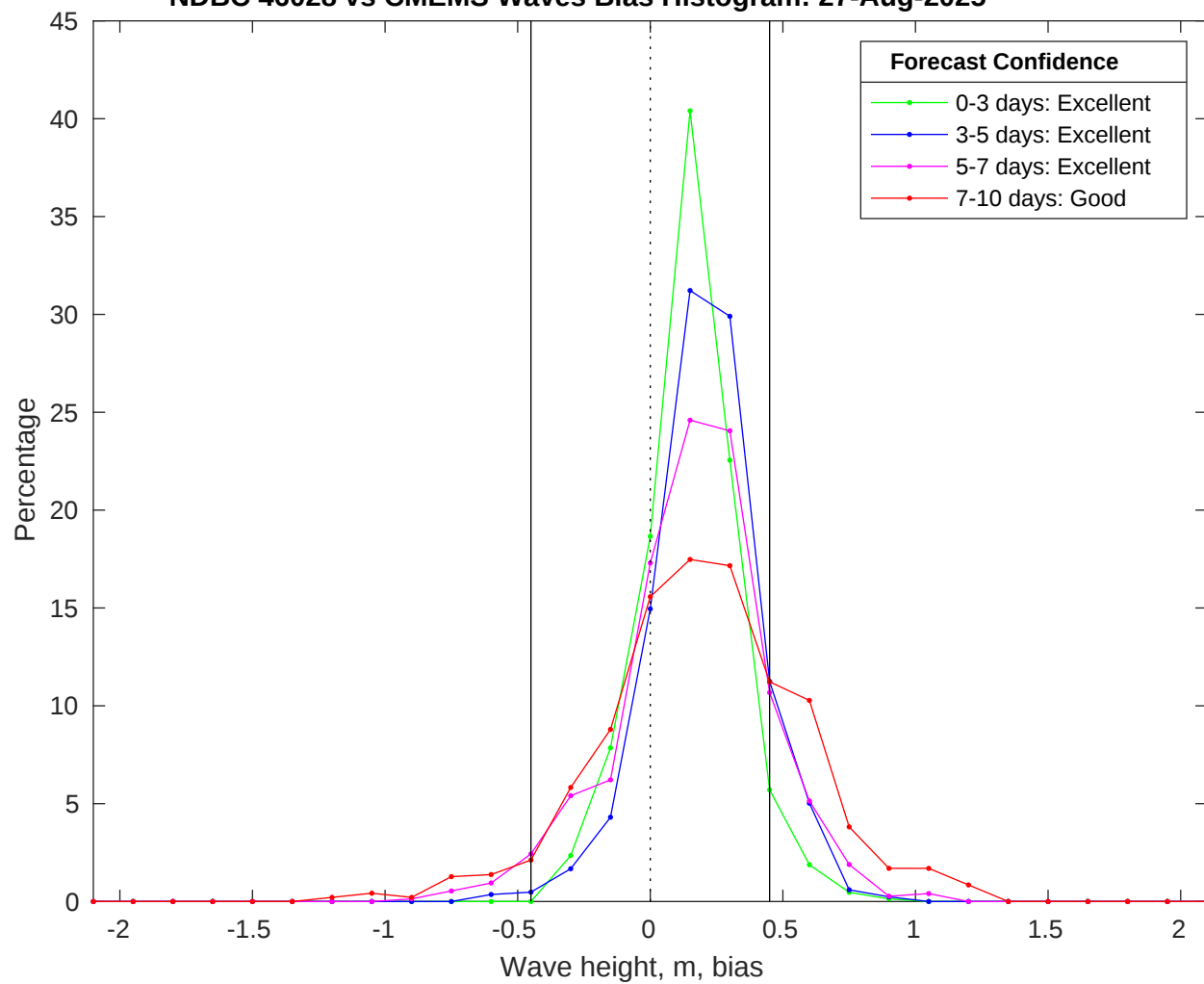
NDBC 46028 vs CMEMS Waves Bias Histogram: 27-Aug-2025
