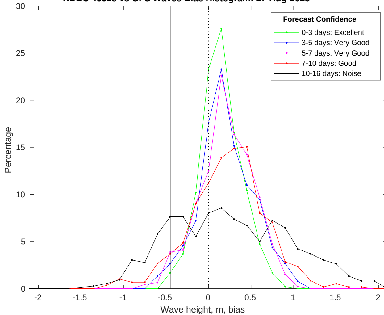
NDBC 46028 vs GFS Waves Bias Histogram: 27-Aug-2025
