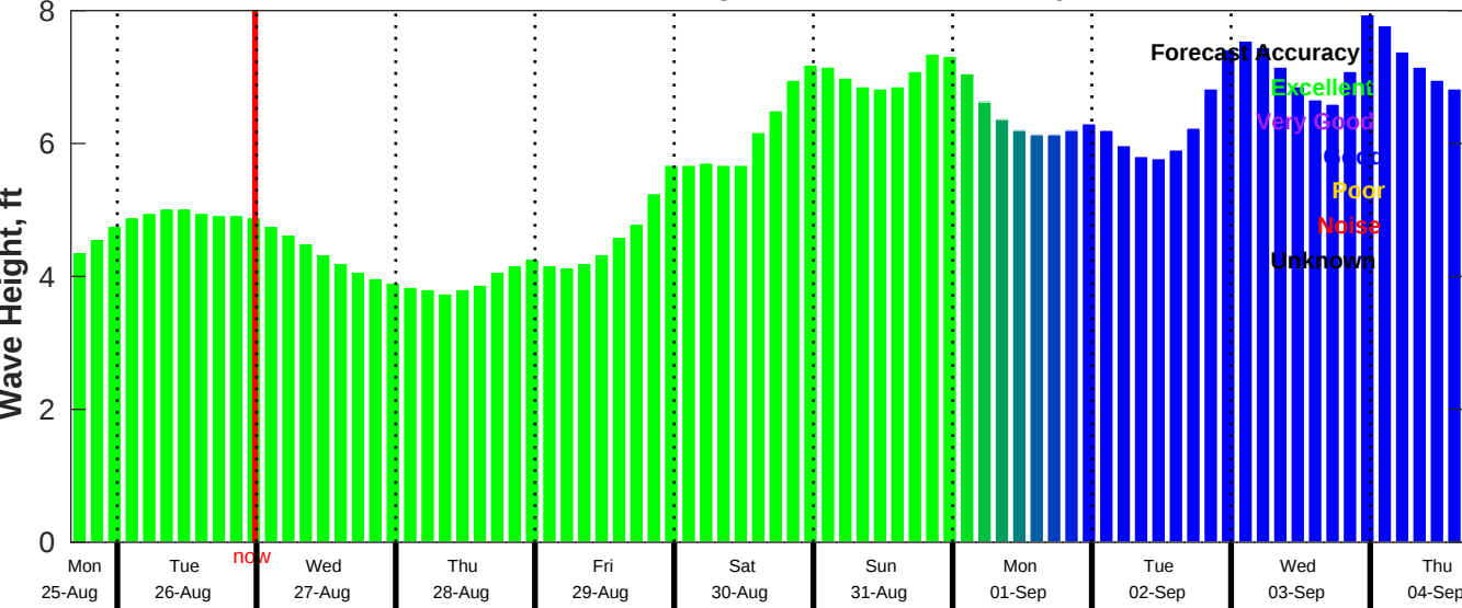
CMEMS Wave Forecast for NDBC 46028 from 25-Aug-2025 16:00:00 to 04-Sep-2025 16:00:00
