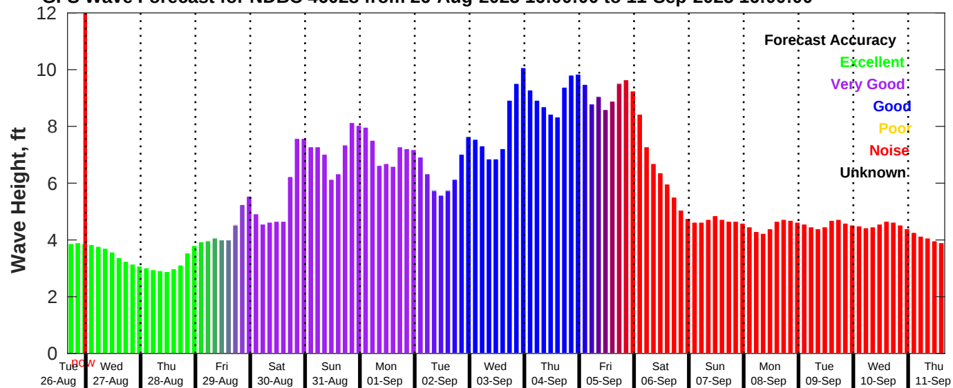
GFS Wave Forecast for NDBC 46028 from 26-Aug-2025 16:00:00 to 11-Sep-2025 16:00:00
