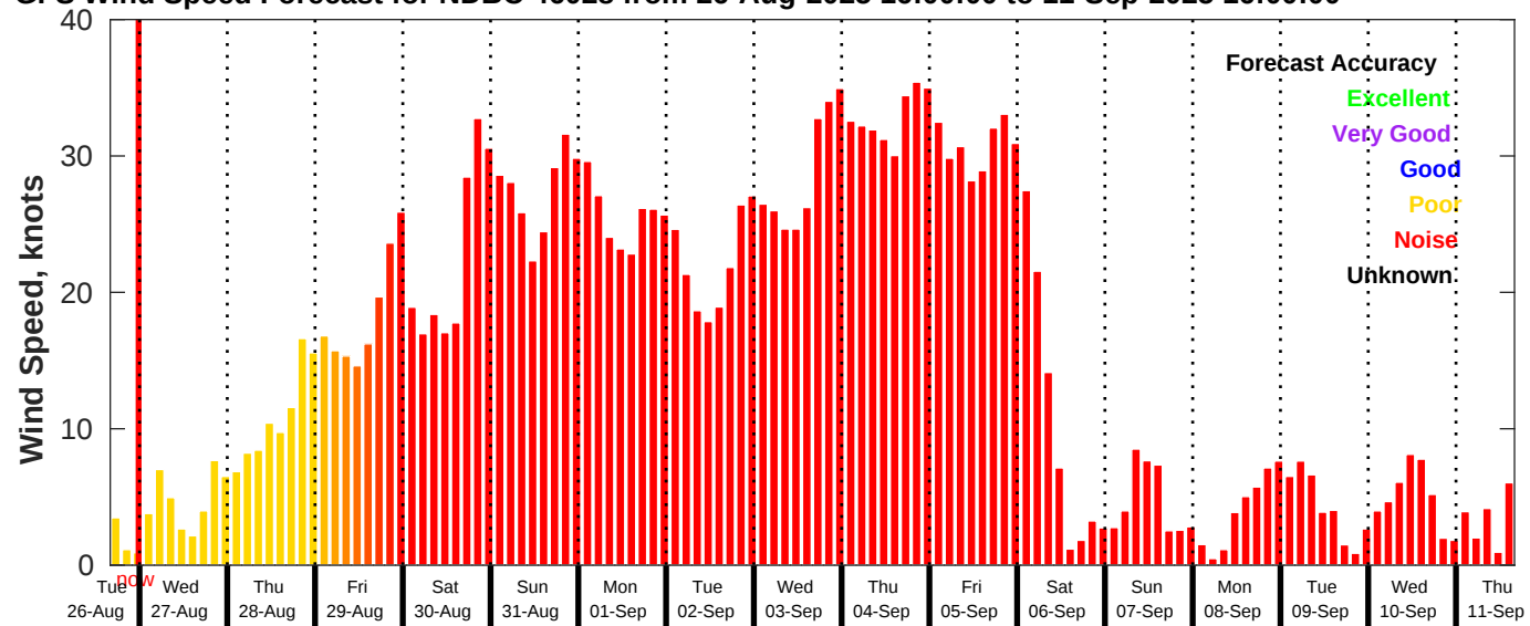
GFS Wind Speed Forecast for NDBC 46028 from 26-Aug-2025 16:00:00 to 11-Sep-2025 16:00:00
