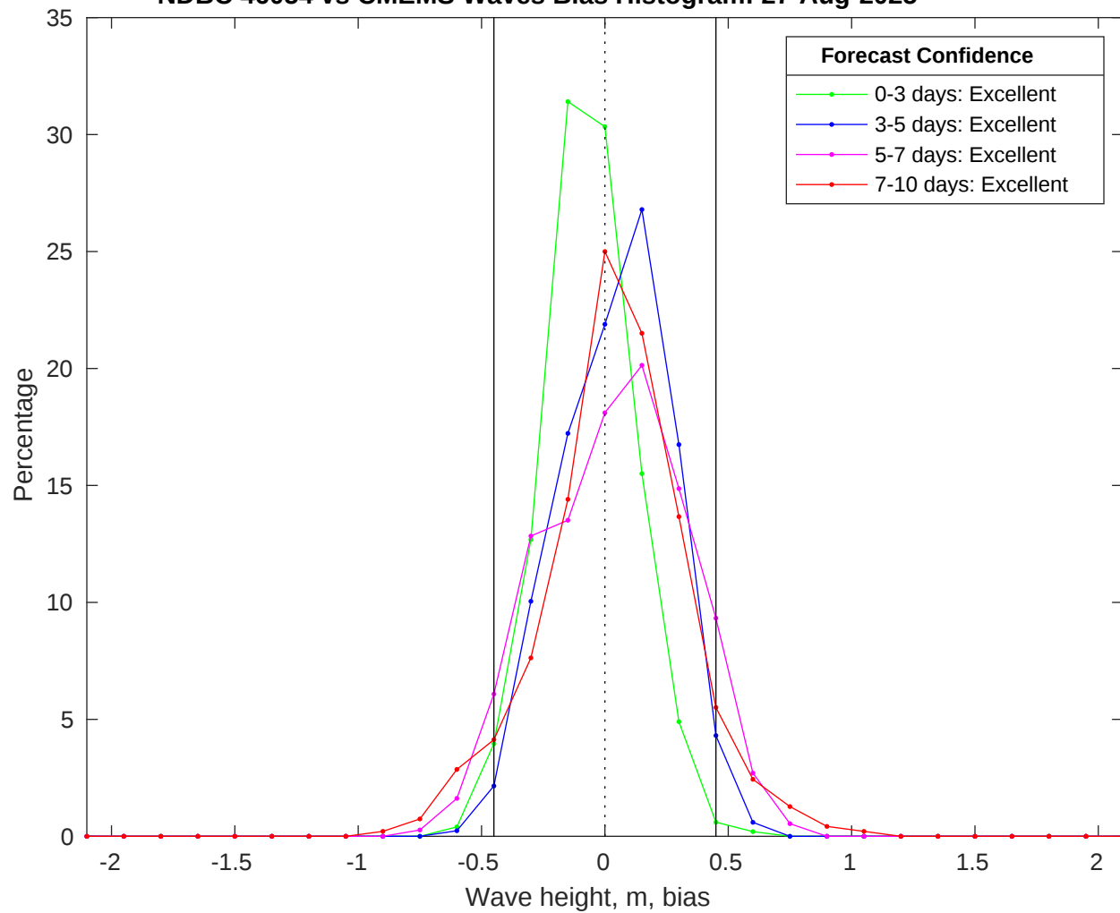
NDBC 46054 vs CMEMS Waves Bias Histogram: 27-Aug-2025
