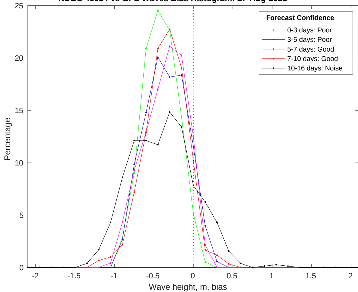
NDBC 46054 vs GFS Waves Bias Histogram: 27-Aug-2025
