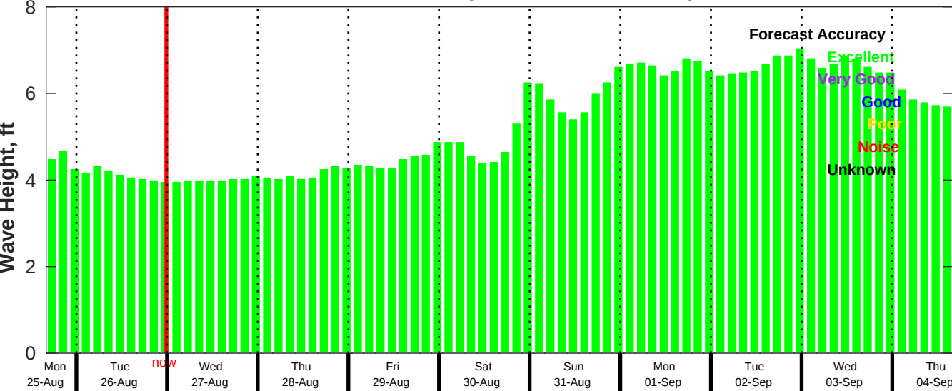
CMEMS Wave Forecast for NDBC 46054 from 25-Aug-2025 16:00:00 to 04-Sep-2025 16:00:00
